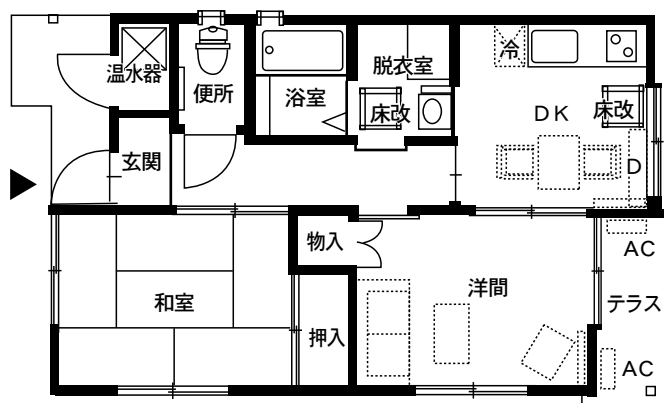
すずほ (45.94㎡)
